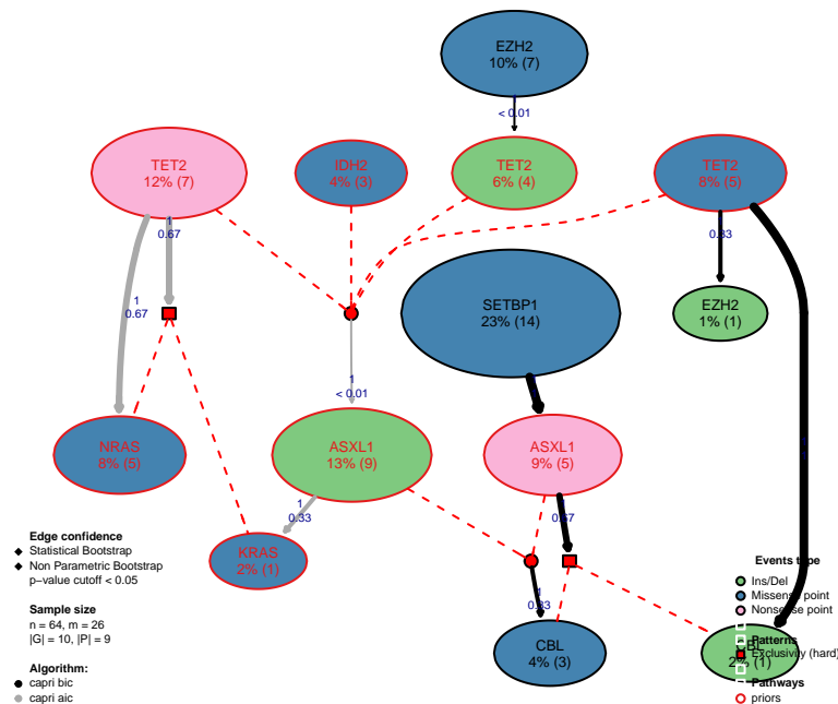
Figure 13: aCML model reconstructed by CAPRI with AIC/BIC as regularizers and annotated with both non-parametric and statistical bootstrap scores Edge thickness is proportional to the non-parametric scores.
