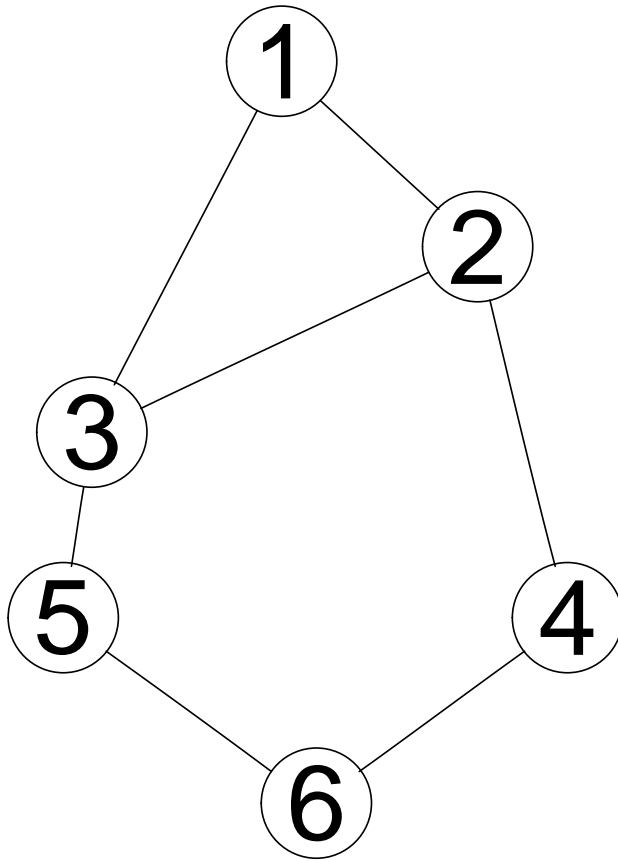
Figure 14: K-cliques Example.
