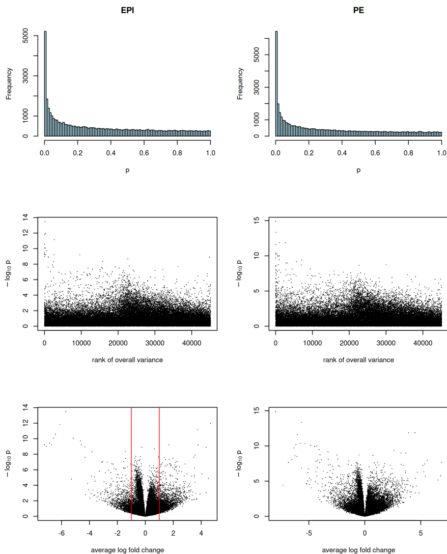
Figure 30: Differentially expressed genes between FGF4-KO and WT (EPI, PE) at E3.5. The upper panels show the histograms of p -values, middle panels the scatter plots of rank of overall variance ( r_{kv} ) versus -\log_{10} p , lower panels \log_2 fold-change versus -\log_{10} p ("volcano plots"). The red lines indicate possibly useful fold change thresholds.
