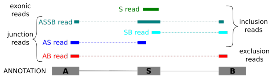
Figure 2: Different categories of reads. In this figure, we show an example of an alternative skipped exon. AS reads correspond to reads spanning the junction between the excluded sequence and its left flanking exon, SB to reads spanning the junction between the excluded sequence and its right flanking exon, ASSB to reads spanning the two inclusion junctions, S to reads entirely included in the alternative sequence and AB to reads spanning the junction between the two flanking exons. S reads correspond to exonic reads and all other categories of reads represented here correspond to junction reads.
