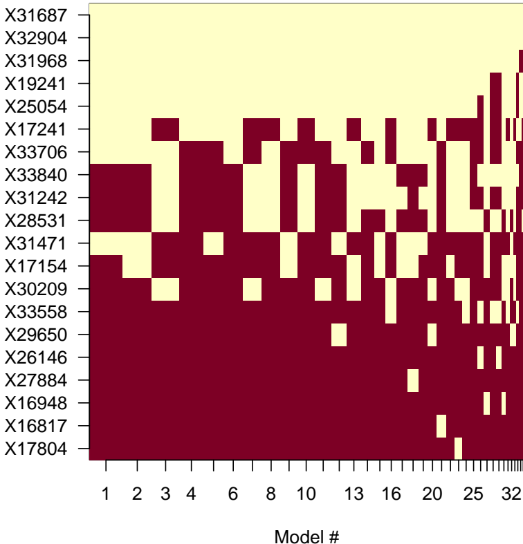
Figure 1: An image plot showing the selected genes and models.
