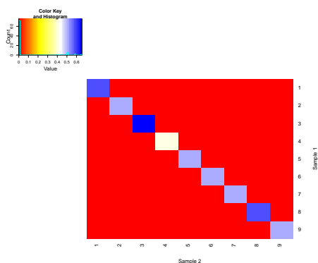
Figure 5: Heatmap of the FR statistics p-values comparing Sample 1 with Sample 2. The p-values of the matched populations (in the diagonal) are significantly larger than the mismatched cell populations.
