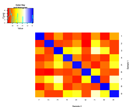
Figure 4: Heatmap comparing cell populations between Sample 1 and Sample 2. The matched populations (in the diagonal) are quantified with significantly smaller FR statistic values than the mismatched populations (correspond to off-diagonal entries). The (i,j) cell contains the FR statistic of comparing the Sample 1 i -th cell population with Sample 2 j -th cell population.
