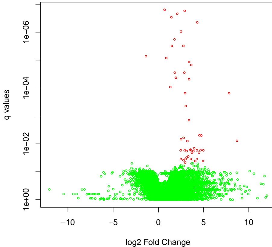
Volcano Plot
