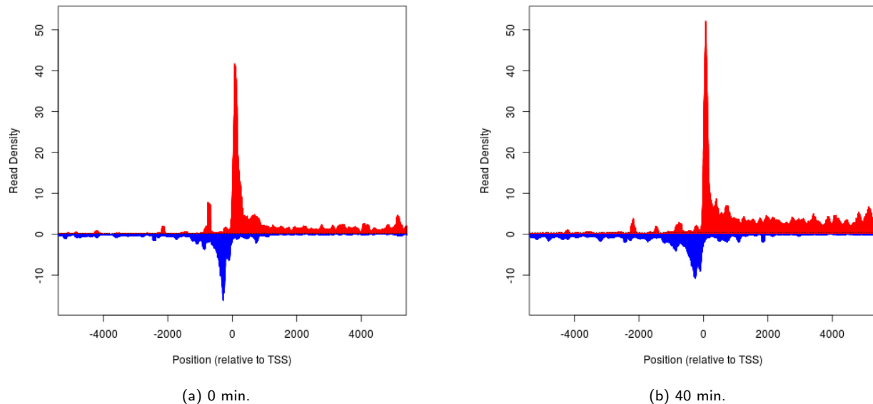
Figure 4: Metagenes
