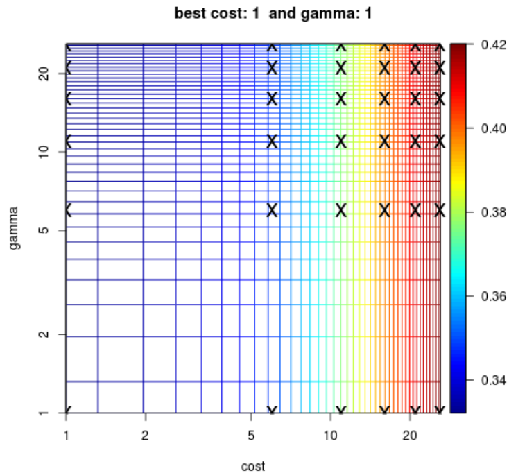
Figure 1: Error prediction by SVM linear kernel method. We use the same plot for linear and radial kernel mcTune optimization but gamma does not give any information for the linear kernel.
